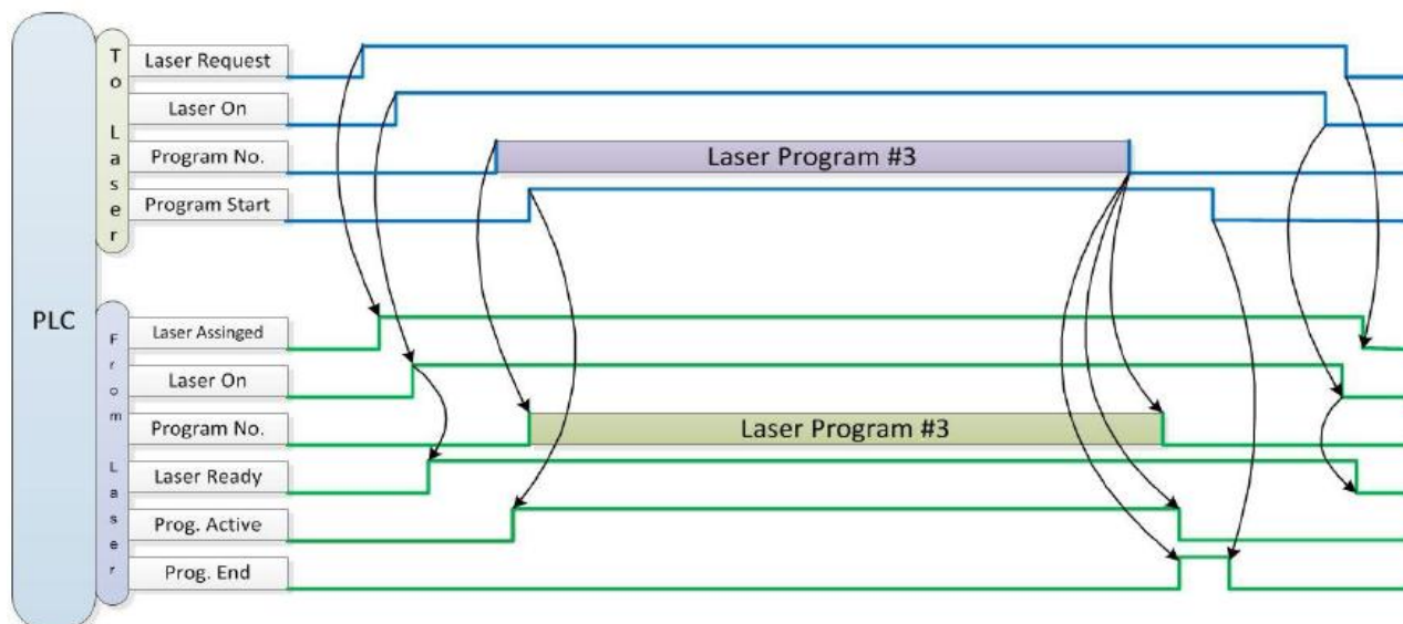
Figure 26 Timing diagram
