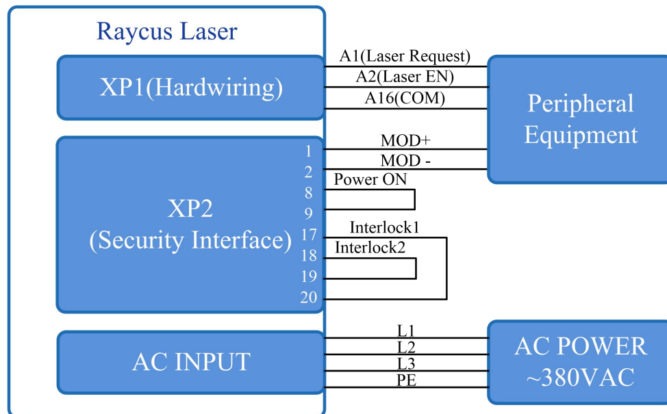
Figure 18 Wiring diagram of power internal control and laser emission external
