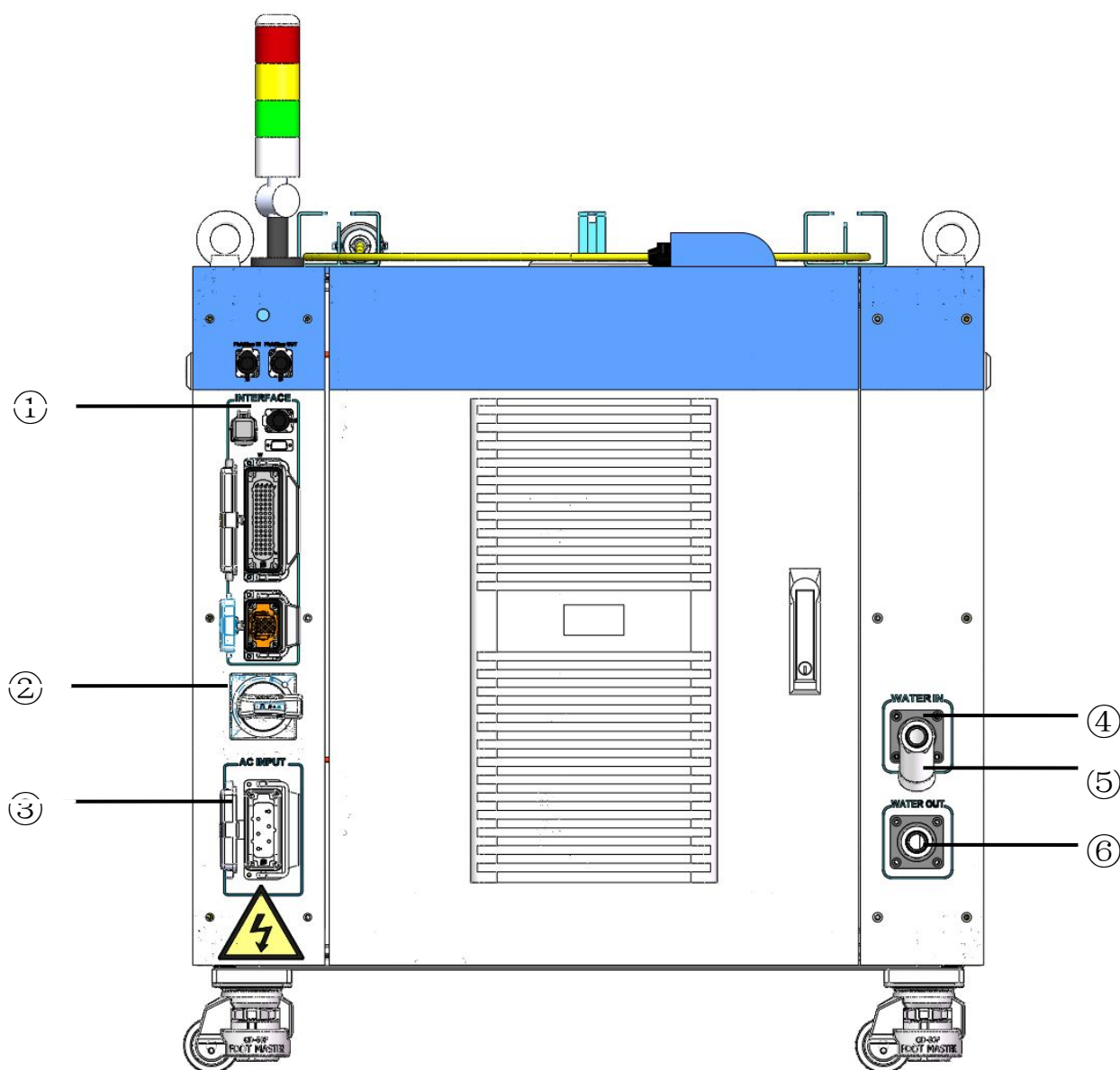
Figure 7 Rear view of product panel
