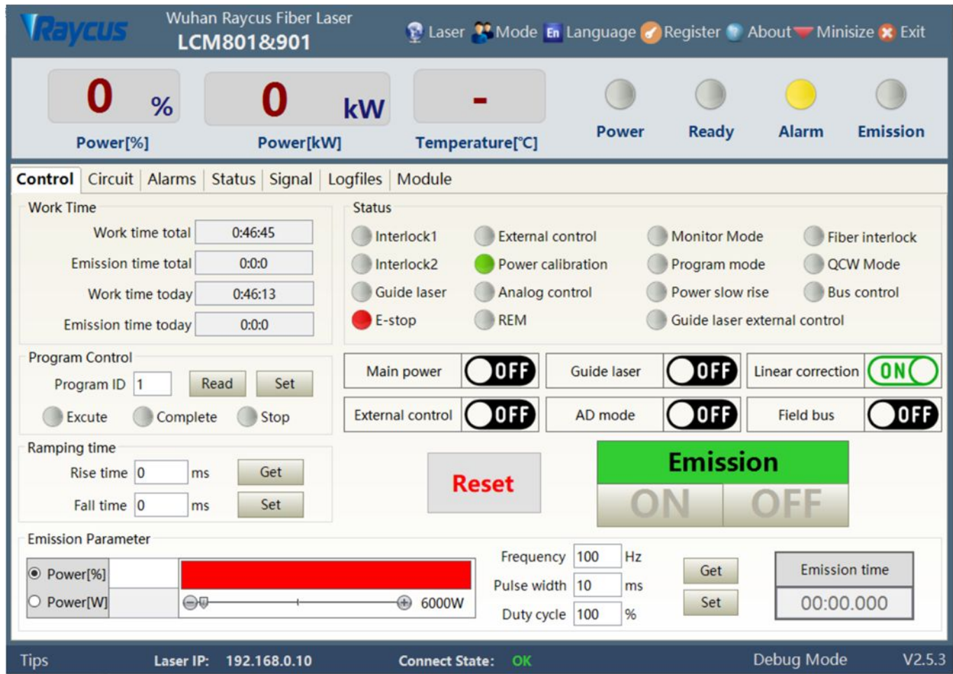
Figure 21 Raycus software’s main menu
